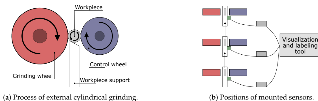
Figure 3. (a) Basic parts of a centerless external grinding machine. (b) Positions of mounted sensors at the grinding machine in our study. Three separate grinding/control wheel pairs allow for efficient machining of complex workpieces with successive processing steps.
