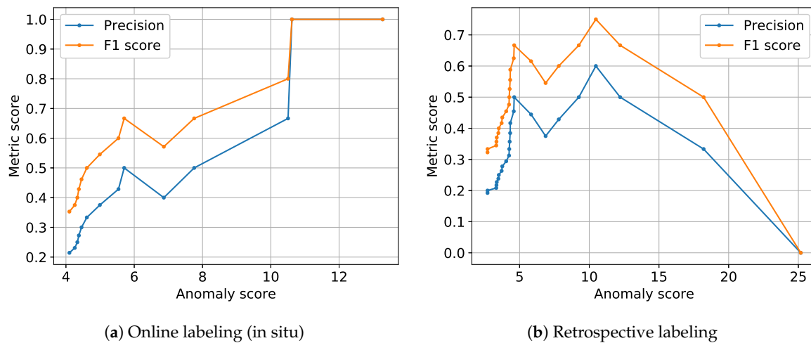
Figure 8. Dependency of metric scores (precision, F1 score) for label feedback on the height of anomaly scores of the NC model (cf. Assumption 2a): For online labels (a), the dependency between likelihood of confirmation of proposed anomalies and height of anomaly scores is clearer than during retrospective annotation (b).
