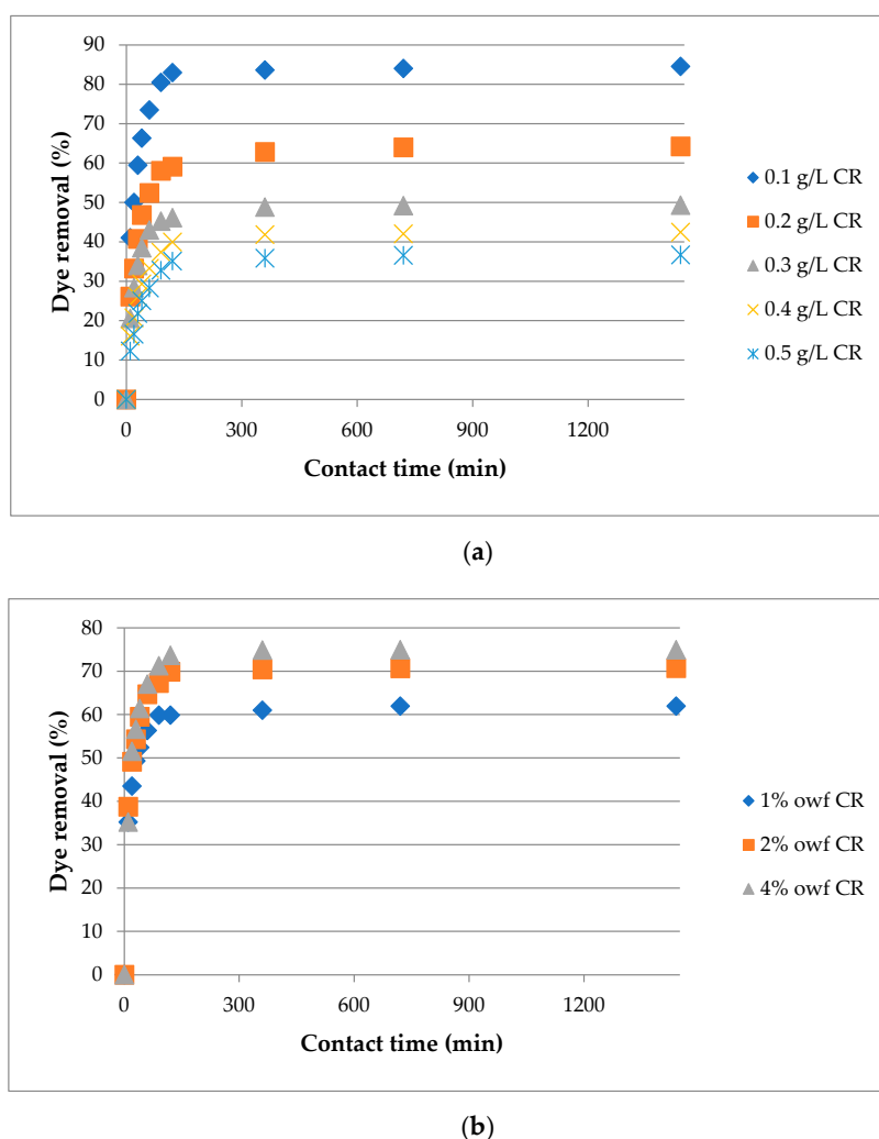
Figure 10. Dye removal vs. contact time of: (a) alkaline scoured S20_70/30 rice husk (adsorption conditions are 0.1 to 0.5 g/L Congo red (CR), 25 °C, 10 g/L rice husk) and (b) ERH (adsorption conditions are effluent from dyeing cotton with 1%, 2% and 4% (owf) initial concentration of CR, 90 °C initial temperature and 10 g/L rice husk).
