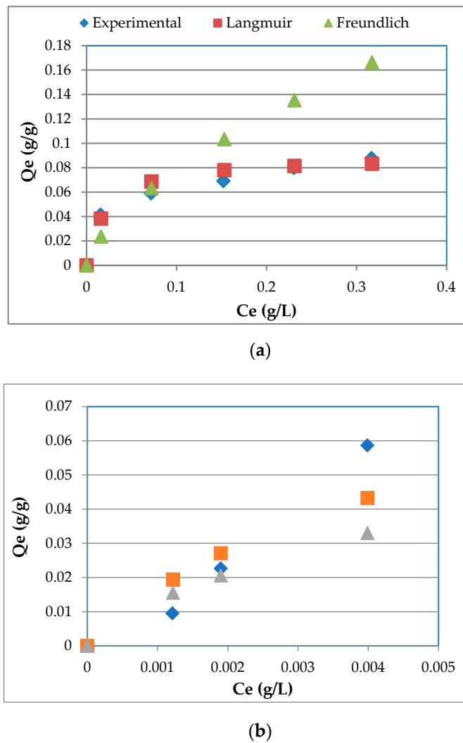
Figure 11. Equilibrium curves for sorption of Congo red onto (a) S20_70/30 and (b) ERH.
