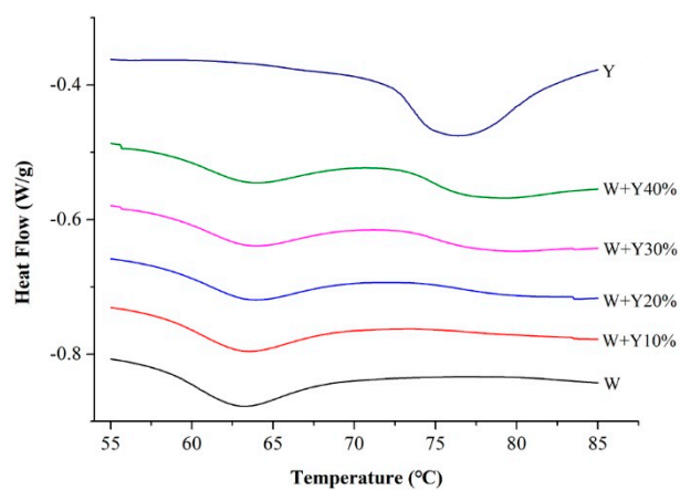
Figure S1. Differential scanning calorimetry (DSC) traces of the gelatinization parameters of control wheat flour (W) and yam powder (Y) and wheat flour-yam powder mixtures at 10% to 40%.
