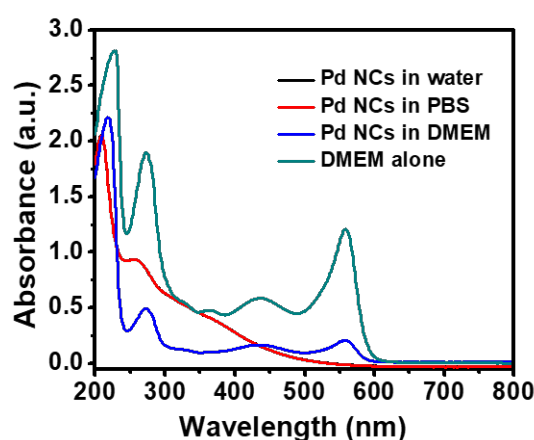
Figure S1. Absorption spectra of Pd NCs in various biological media medium.
