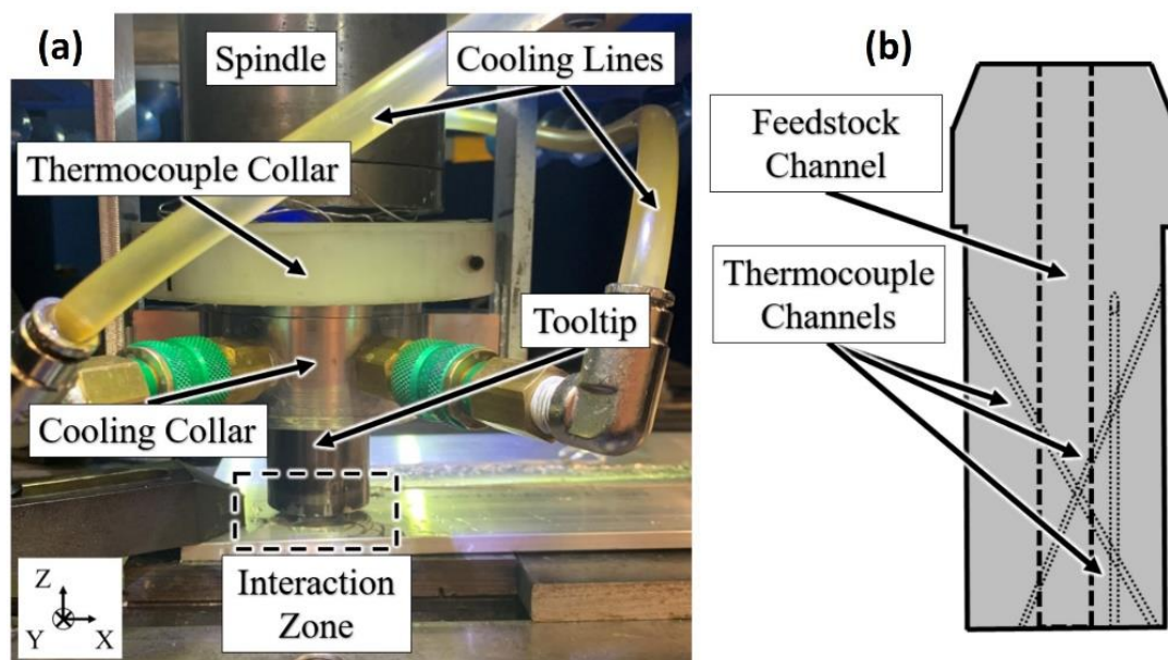
Figure 8. The modified setup showing (a) thermocouple and cooling collars, and (b) thermocouple channels (licenced under CC BY 4.0) [12].
