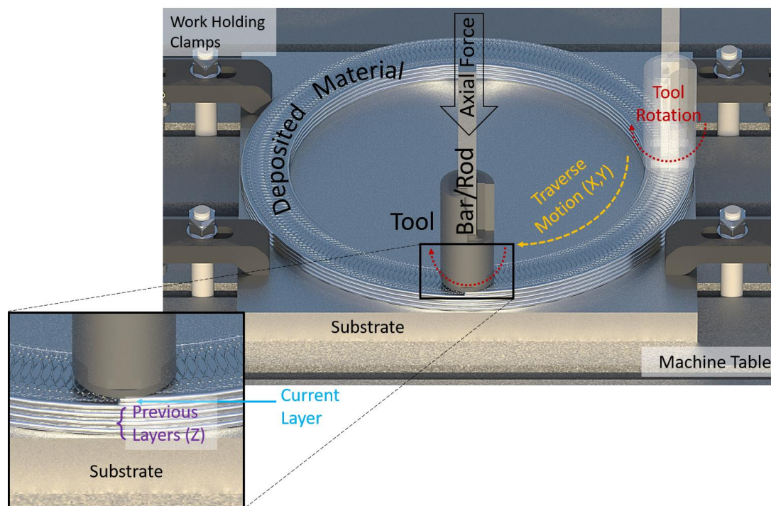
Figure 1. Schematic illustration of the AFSD process.
