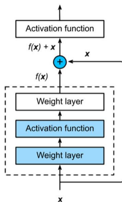
Figure 5. Residual learning: a building block.
