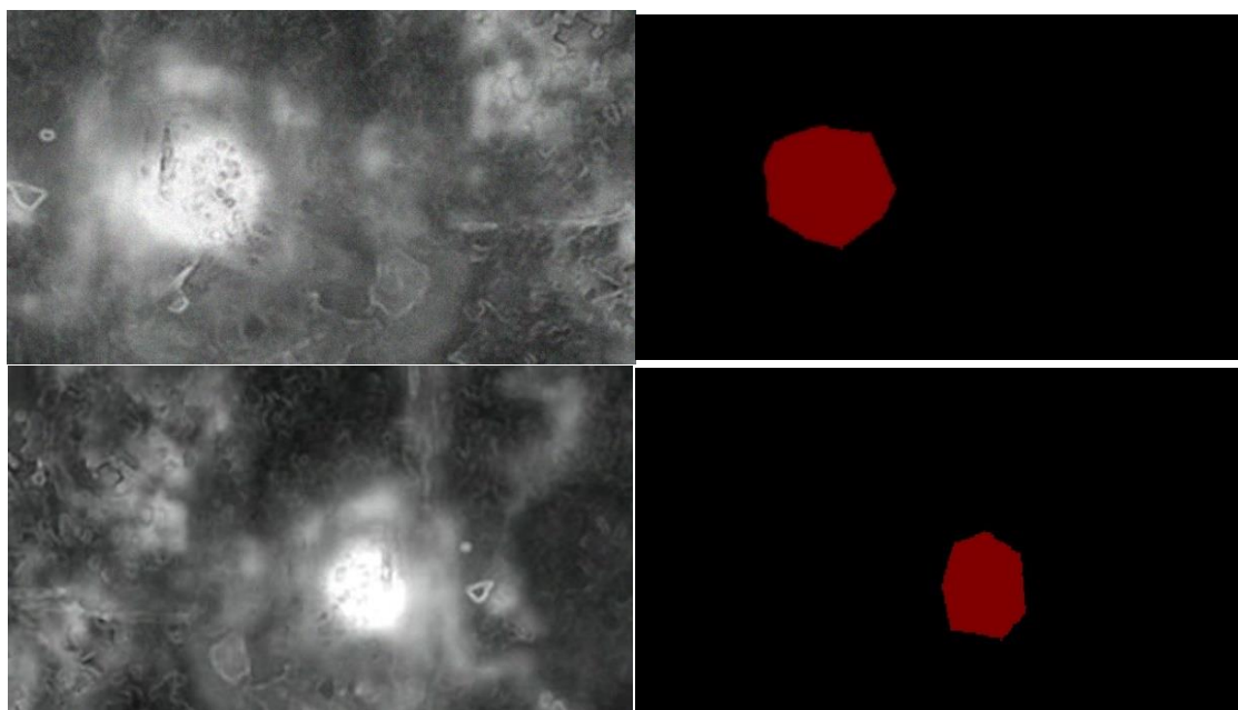
Figure 3. Adaptive thresholding using Otsu’s method—thermal image acquired from DJI drone ( left ) and segmentation map ( right ), where (black) red corresponds to pixels in which fire was (not) detected. Setup shown above was for experimental test fire, as shown in Figure 1.
