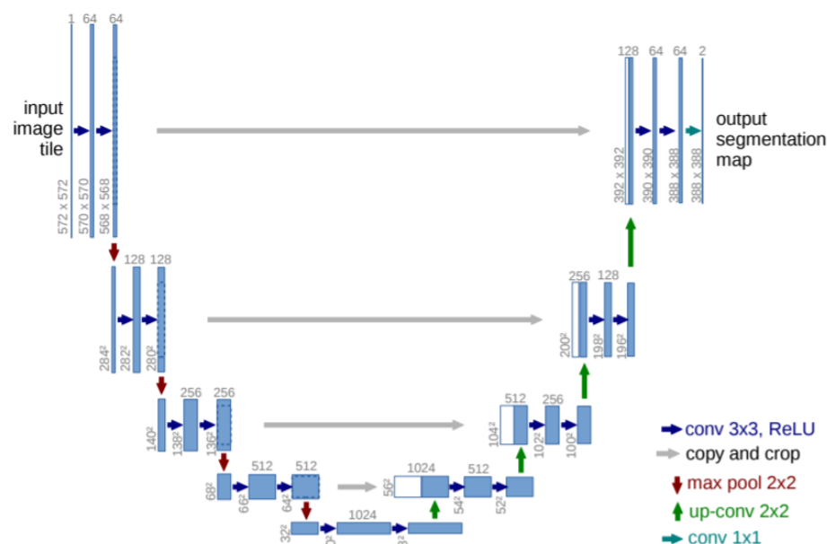
Figure 4. Overview of UNET architecture [20].
