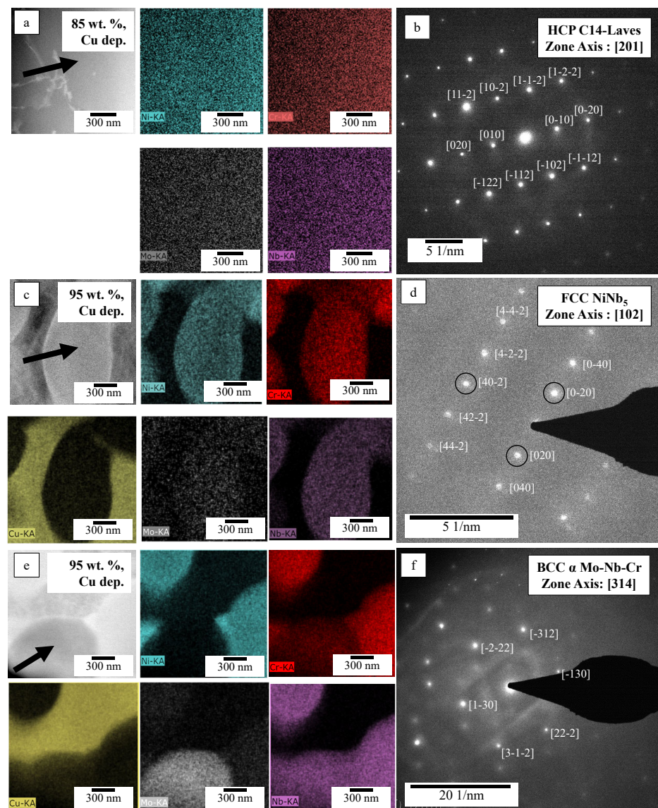
Figure 4. STEM-EDS maps showing the (a) HCP C14-Laves in the 85 wt.% GRCo42 Cu-depleted region along with (b) the corresponding SAD pattern in the [201] zone axis, (c) FCC \text{NiNb}_5 phase in the 95 wt.% GRCo42 Cu-depleted region along with (d) the corresponding SAD pattern in the [102] zone axis, and BCC \alpha Mo-Nb-Cr phase in the 95 wt.% GRCo42 Cu-depleted region with (e) the corresponding SAD pattern in the [314] zone axis. The arrows in (a,c,e) point to the location of SAD pattern collection. The circled spots in (d) are attributed to double diffraction.
