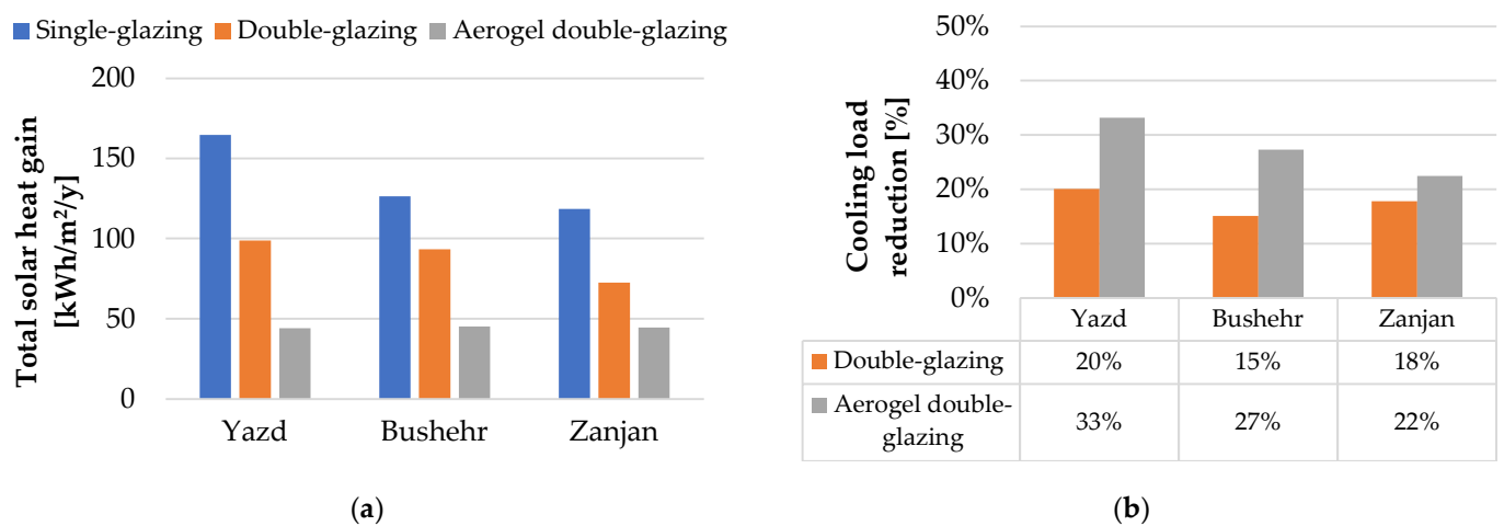
Figure 2. Simulated results for school buildings in Yazd, Bushehr, and Zanzan: (a) total solar gain for the investigated window configurations; (b) cooling load reduction of double-glazing and aerogel configurations compare to the single-glazing pane.
